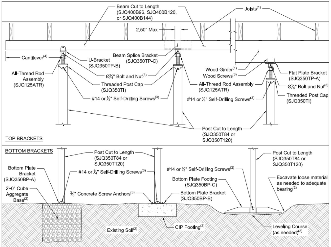
Figure 1 Continued– SmartJack System Assemblies and Components
