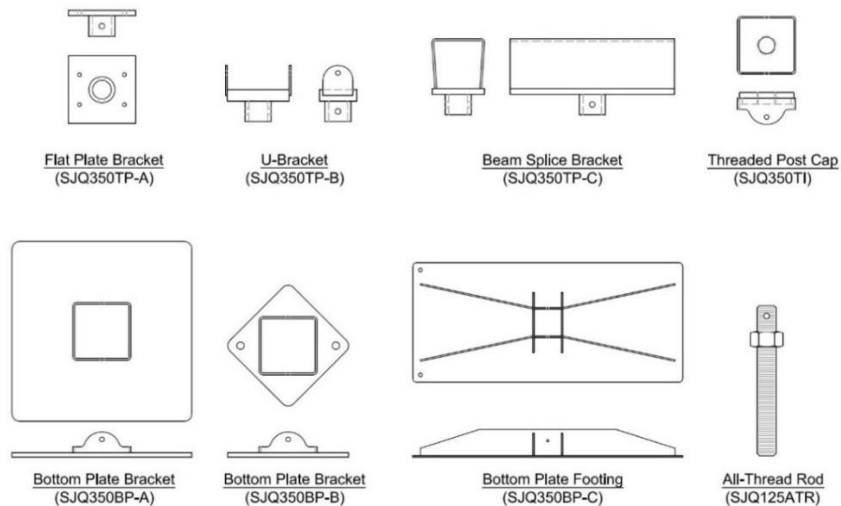
Figure 1 – SmartJack System Assemblies and Components
