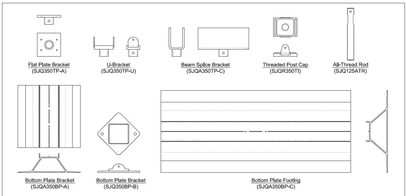
FIGURE 1 – SmartJack System Assemblies and Components (continued on next page)
